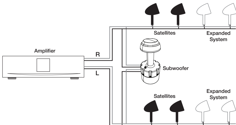
Figure 9: Wiring Setup
