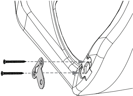
Figure 7b: Flip/Re-attach Keyway
