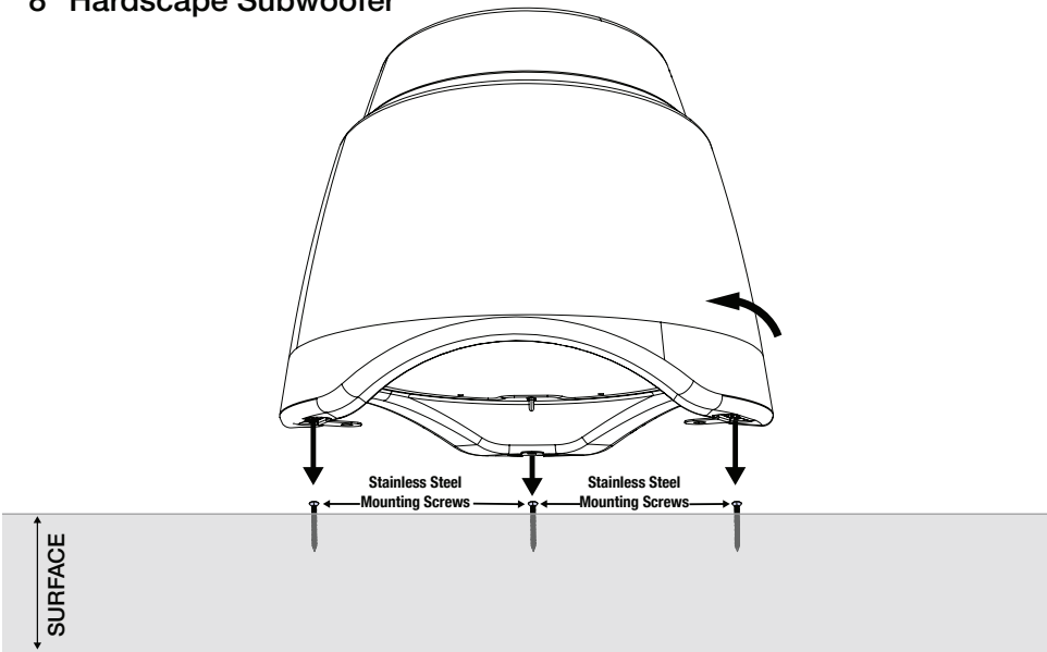
Figure 6: Secure Subwoofer
