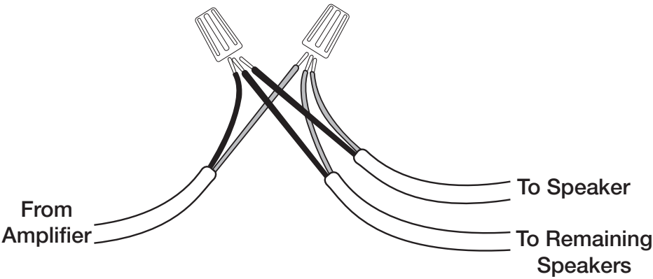
Figure 10: Wiring Bundle
