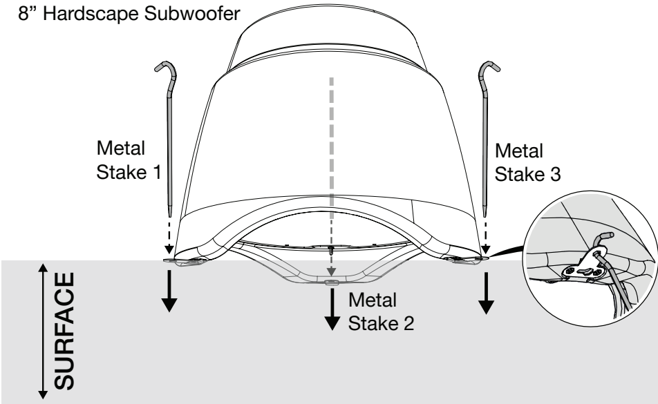
Figure 8: Secure Subwoofer (Stakes)
